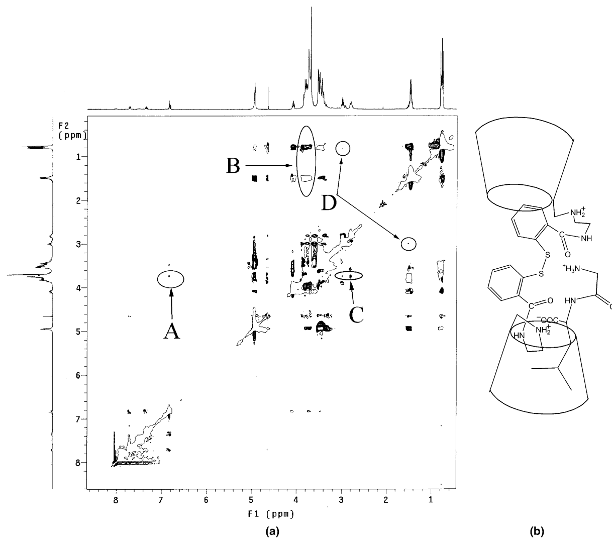
Figure 3. ROESY spectrum of 1/Gly-Leu system ( [1] = [\text{Gly-Leu}] = 2.0 \text{ mM} ) in pD 7.20 buffer solution.
