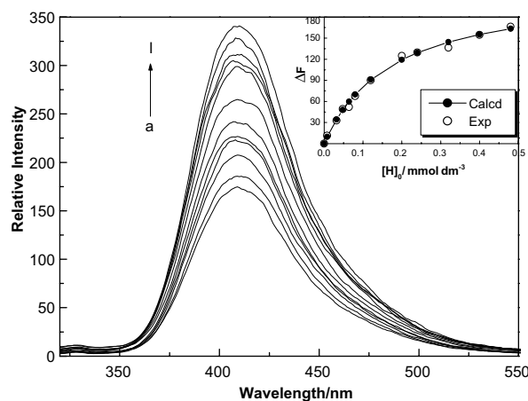
Figure 2. Fluorescence spectral changes of bis( \beta -CyD) 1 (8 \mu M) and the nonlinear least-square analysis (inset) of the differential intensity ( \Delta F ) used to calculate the complex stability constant ( K_S ) upon addition of Gly-Pro (0–480 \mu M; traces a–l) in an aqueous buffer solution of pH 7.20 at 25 °C; excitation at 295 nm.
