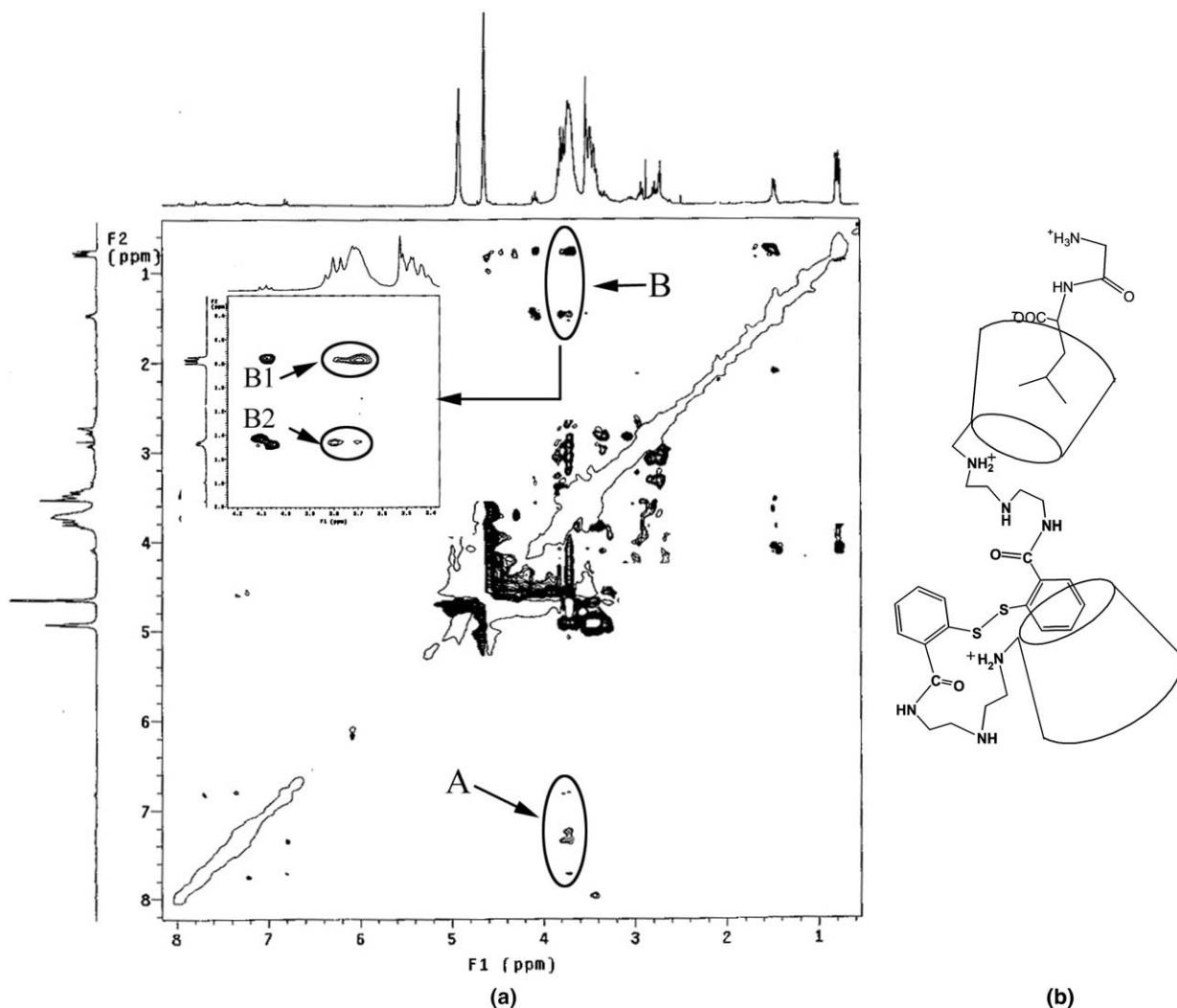
Figure 5. ROESY spectrum of 2/Gly-Leu ([2] = [Gly-Leu] = 2.0 mM) in pD 7.20 buffer.
